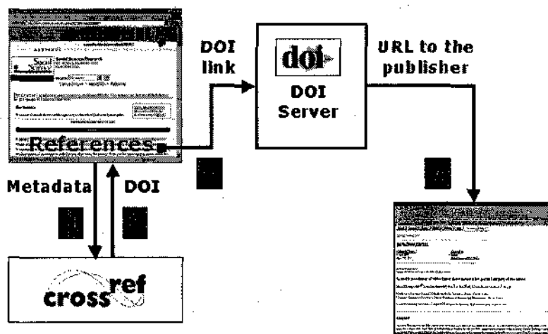
Figure 4: DOI/CrossRef framework
