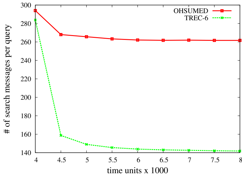
Figure 8.7: Search messages per query for different corpora
