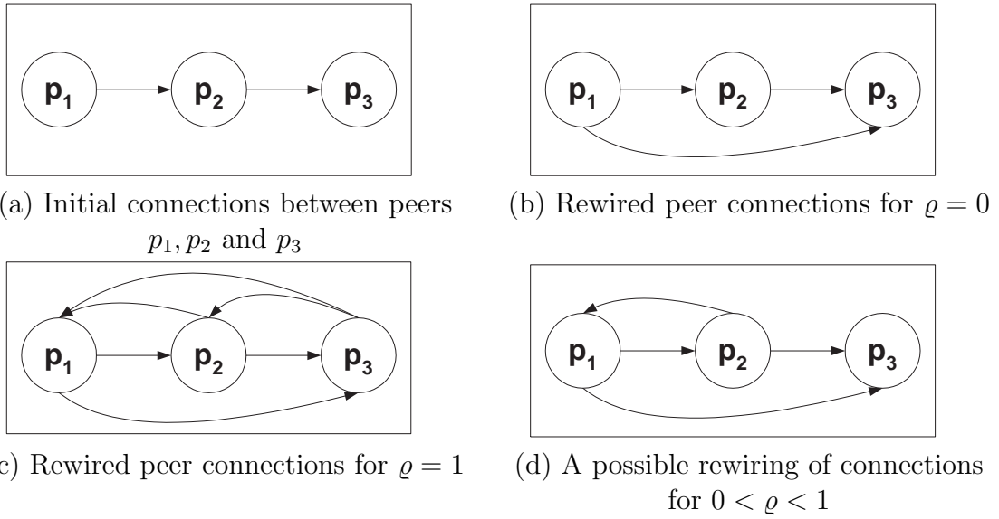
Figure 4.3: An example illustrating the usage of the refinement probability \varrho
