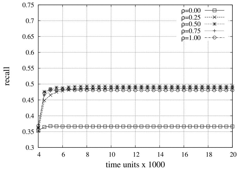
Figure 7.7: Retrieval effectiveness for different values of \rho when using the GW strategy (TREC-6)
