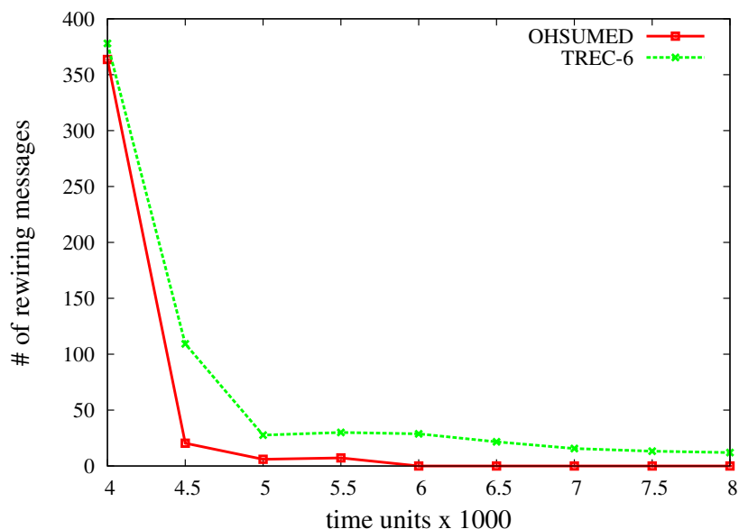
Figure 8.6: Organisation messages for different corpora
