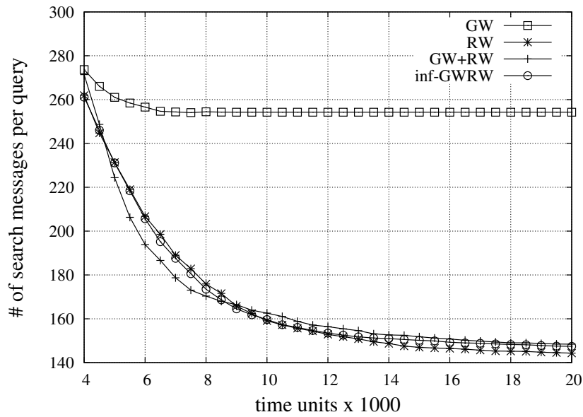
Figure 7.6: Search messages per query for different forwarding strategies (TREC-6)
