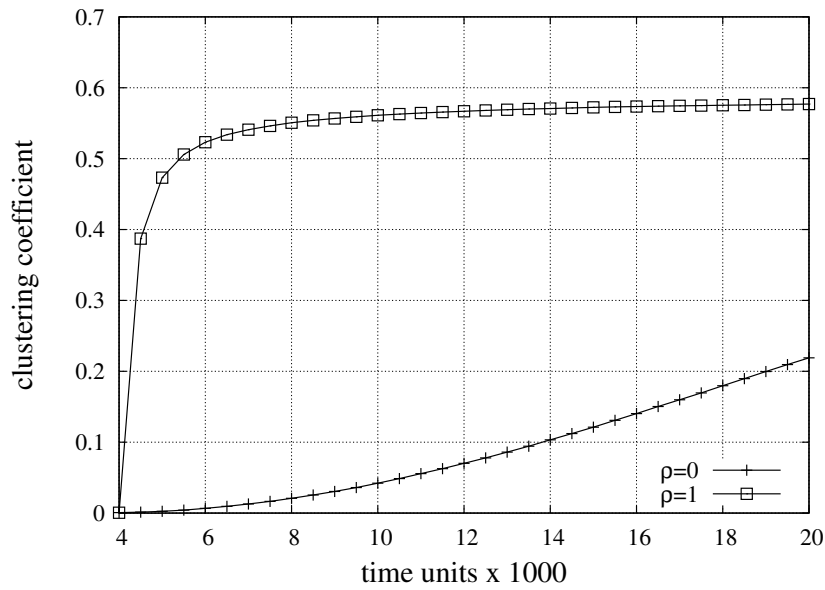
Figure 7.17: Clustering coefficient \bar{c} as a function of time for different values of \varrho
