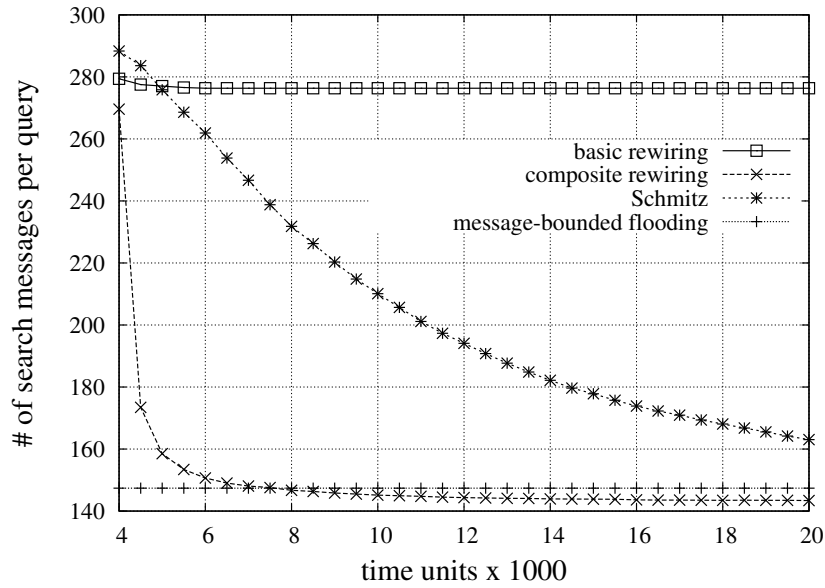
Figure 7.14: Comparison of the communication overhead (in search messages) of different rewiring protocols (TREC-6)
