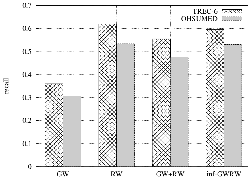
Figure 7.4: Retrieval effectiveness for different forwarding strategies
