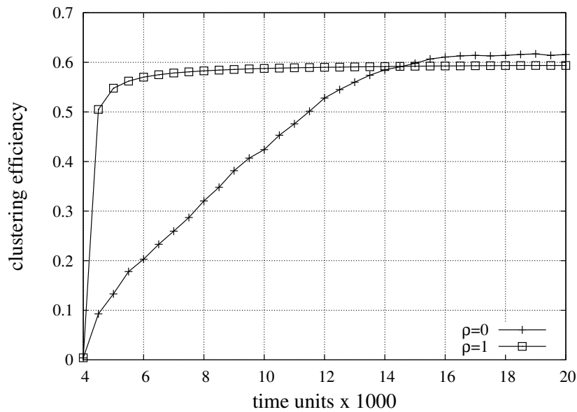
Figure 7.18: Clustering efficiency \bar{k} as a function of time for different values of \varrho
