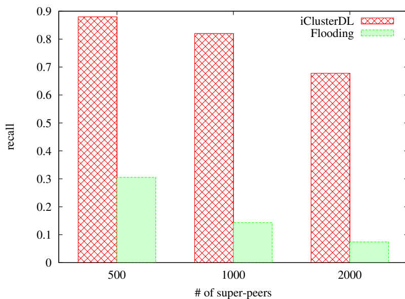
Figure 8.5: Recall for iClusterDL and Flooding using the same number of messages (TREC-6)
