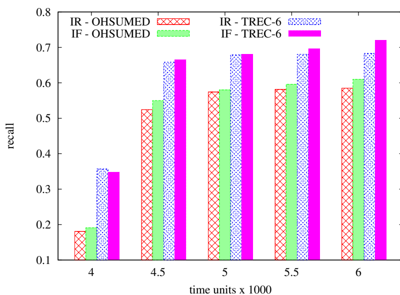
Figure 8.4: Recall over time for both IR and IF scenarios using two real-life corpora
