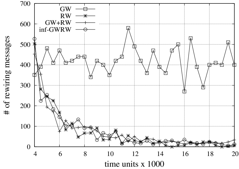
Figure 7.5: Rewiring messages for different forwarding strategies (TREC-6)
