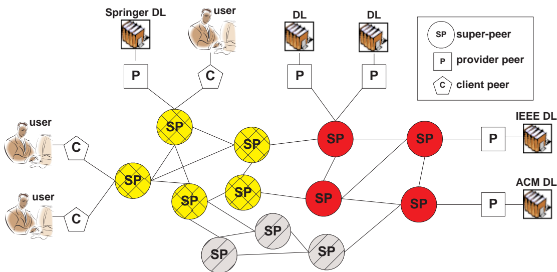
Figure 8.1: A high-level view of the iClusterDL architecture
