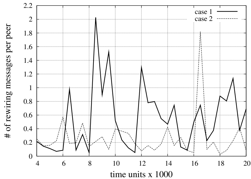
Figure 7.21: Rewiring messages as a function of time
