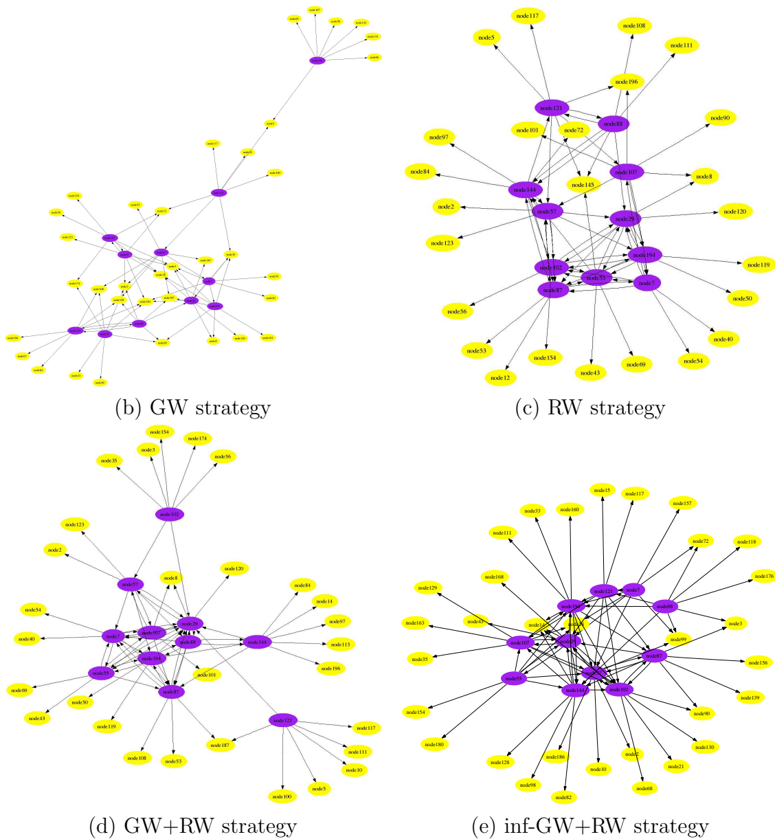
Figure 4.2: Network organisation for different message forwarding strategies
