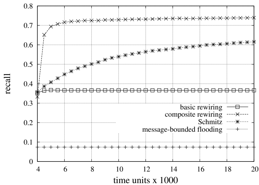
Figure 7.13: Comparison of the retrieval performance of different rewiring protocols (TREC-6)
