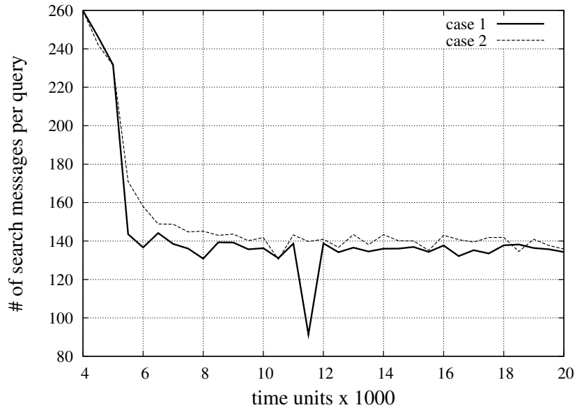
Figure 7.23: Search messages as a function of time
