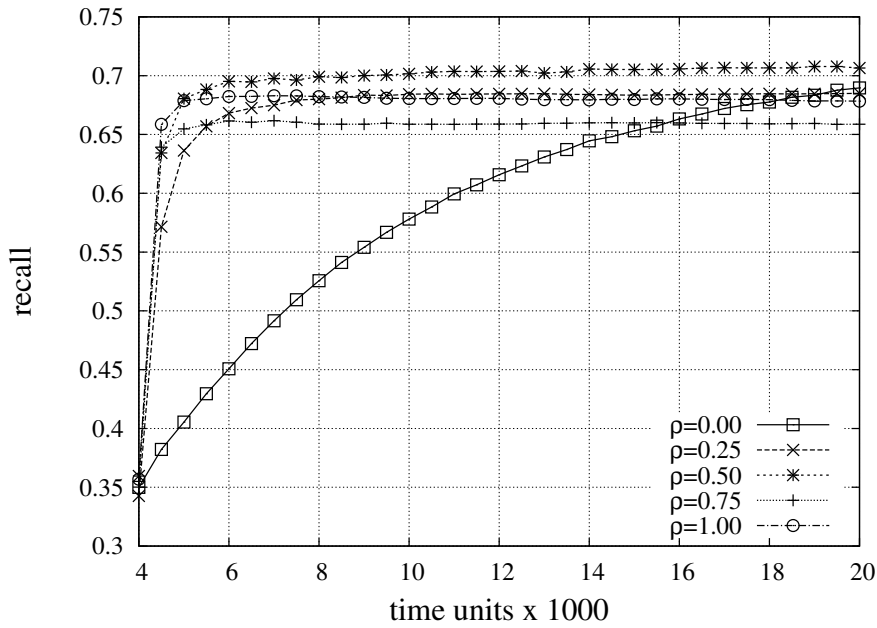
Figure 7.8: Retrieval effectiveness for different values of \rho when using the RW strategy (TREC-6)
