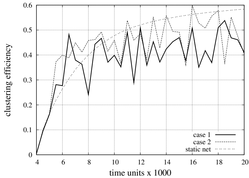
Figure 7.20: Clustering efficiency as a function of time
